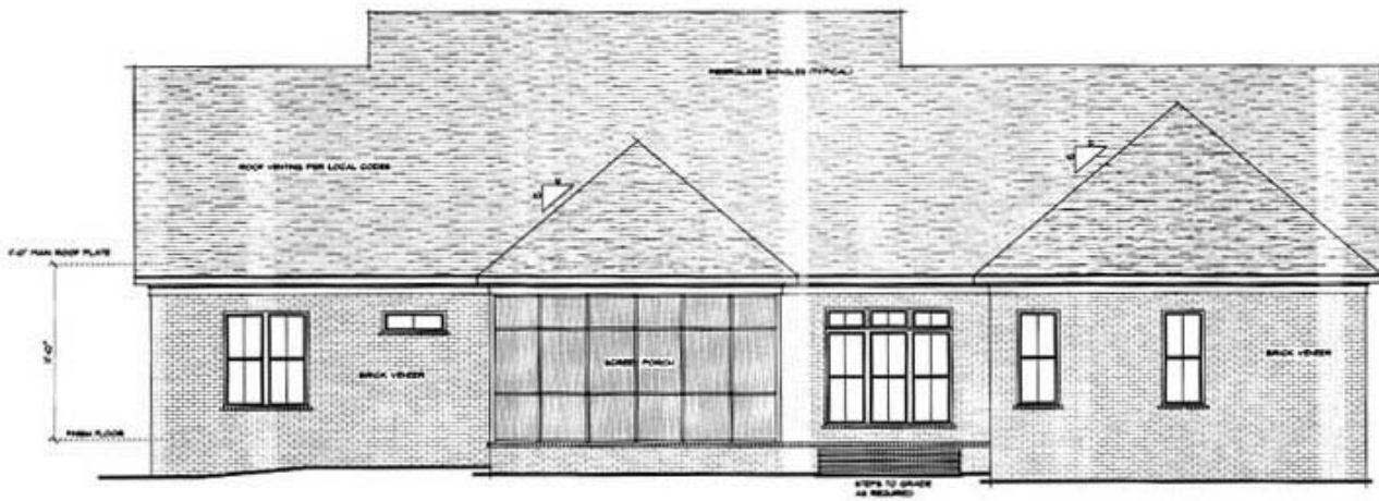
REAR ELEVATION 1/4"
