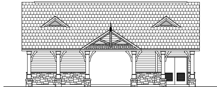
REAR ELEVATION
