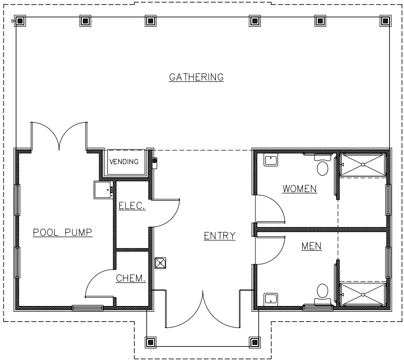
FLOOR PLAN
